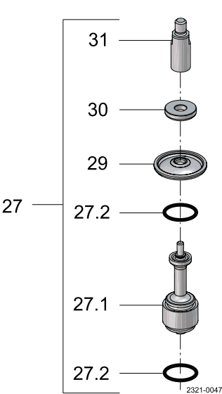
Aseptic plugs - change-over
