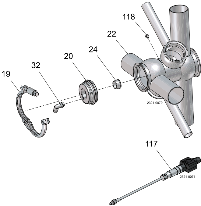
Horizontal mount
