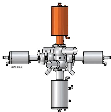
Actuator, primary valves (no seat lift)
