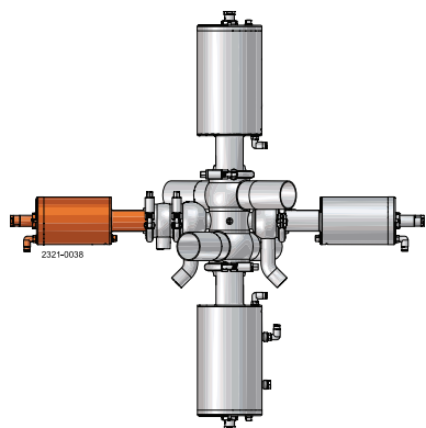
Actuator, secondary valves
