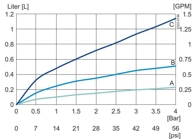
Abbildung 5. Unique Mixproof Process ISO38/DN40/1/2"
